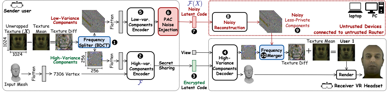
Figure 5. Overview of PRIVATAR avatar reconstruction flow. VR reconstruction is horizontally partitioned into two paths, running on the local device (bottom right) and untrusted devices (upper right red dashed box), separately. Noisy reconstruction is highlighted in red.
