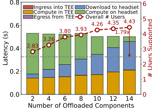
Figure 12. Latency breakdown and overall throughput for CPU with secure memory encryption based secure partial offloading on Quest Pro. Bars decompose end-to-end per-frame latency into Ingress (encrypt & copy into enclave), Compute (CPU inference inside the TEE), Egress (copy out from TEE), Download (return to headset), and Compute on the headset (compute latency of reconstructing local frequency components). The red curve shows the overall throughput (the number of concurrently supported users at 60 FPS). Despite strong confidentiality, limited CPU inference latency restricts its throughput improvement to \sim 1.79\times , which is less than 2.37\times achieved by PRIVATAR.
